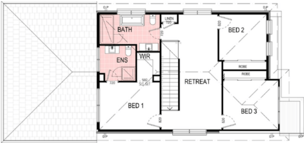
FIRST FLOOR
