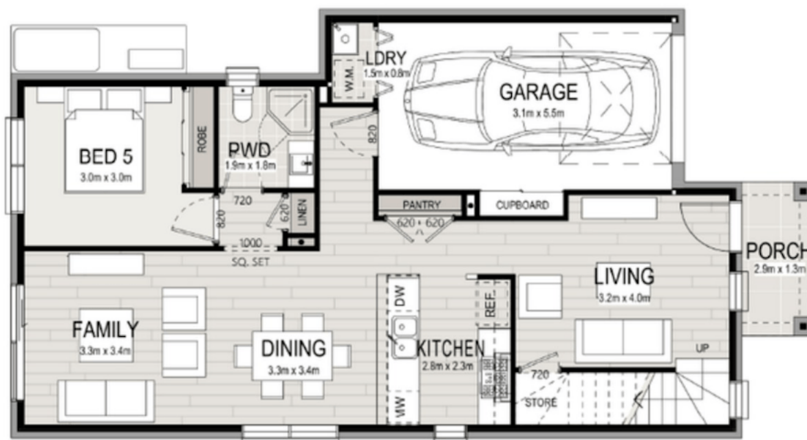
GROUND FLOOR
